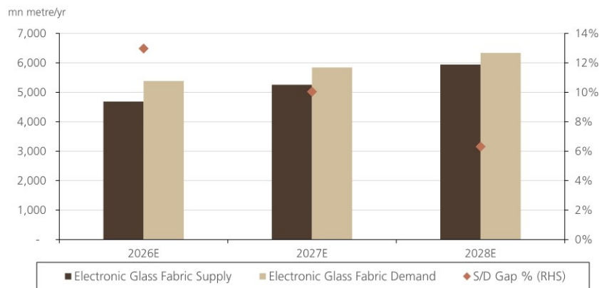
Figure 2: Industry electronic glass fabric (E-glass + speciality/AI) supply/demand forecasts
